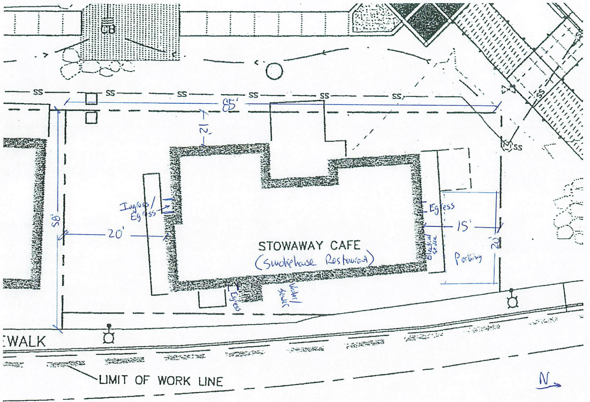
The Smokehouse Plot Plan
